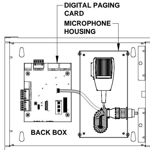
Exhibit 2: Enclosure Layout (Paging Control Card not shown)
