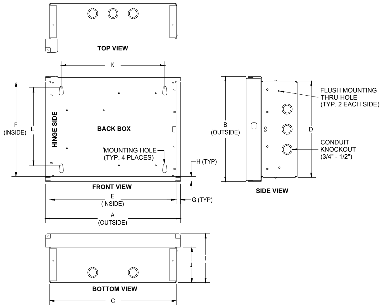
Exhibit 3: Enclosure Dimensions
