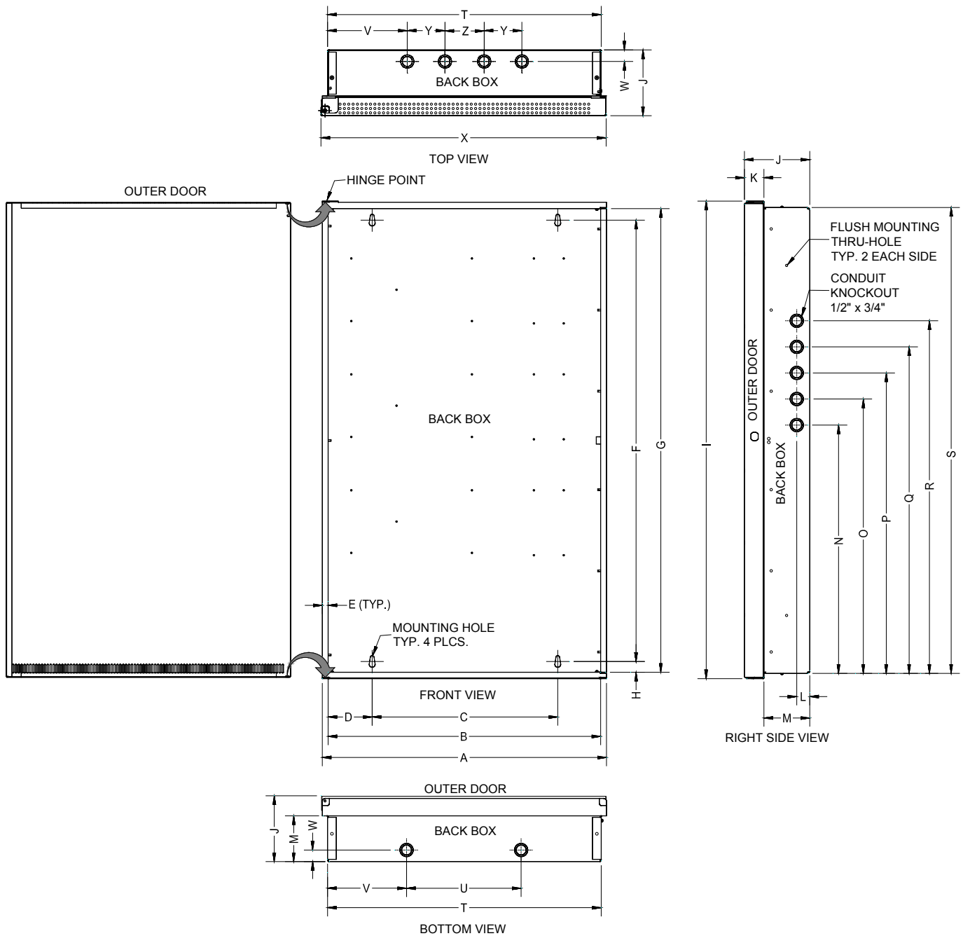
Exhibit 4 3 Slot Enclosure
