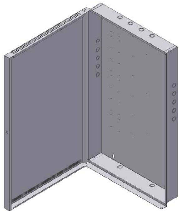
Exhibit 1 3 Slot, Remote Equipment Enclosure
