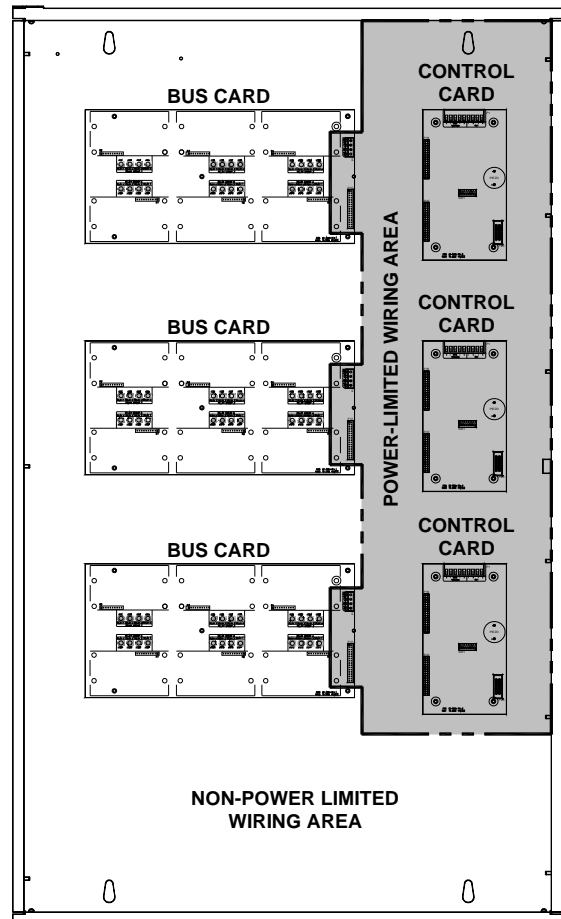
Exhibit 3 Enclosure Wiring Segregation with P/N 10-2777 Relay Control Assembly
