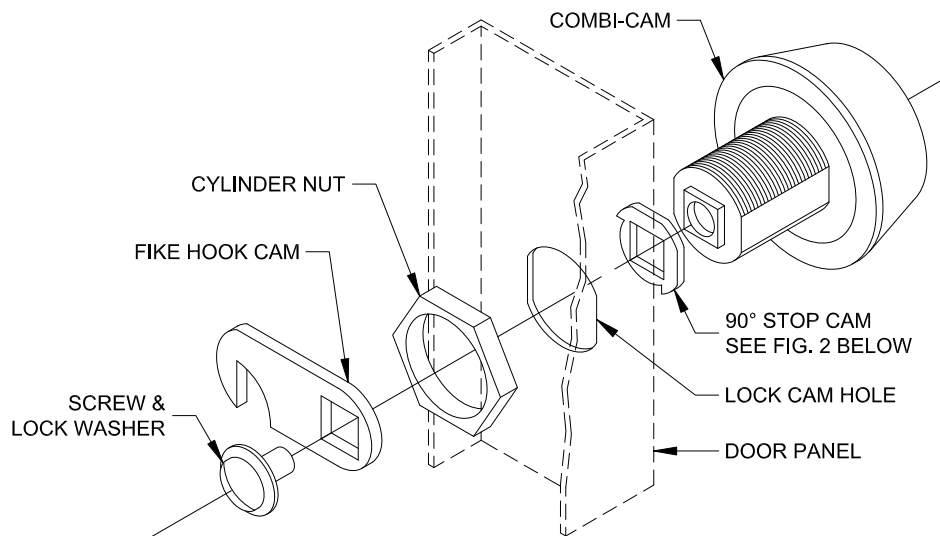
Figure 1 Lock Mechanism Installation
