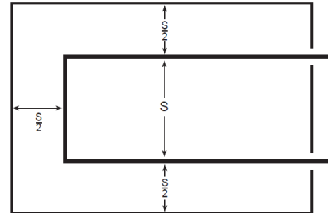
Ceiling of protected area S=Listed spacing. See chart below.
