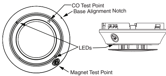
FIGURE 4. CLEANING THE CO DETECTOR
