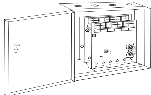
FIGURE 1: FIK-BB-2 CABINET
