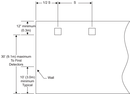
FIGURE 3. MOUNTING LOCATIONS
