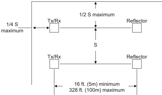
FIGURE 3. MOUNTING LOCATIONS
