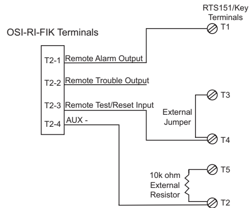
FIGURE 7. OSI-RI TERMINALS
