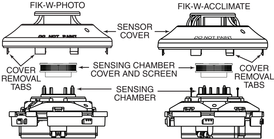
FIGURE 5. DETECTOR COMPONENTS
