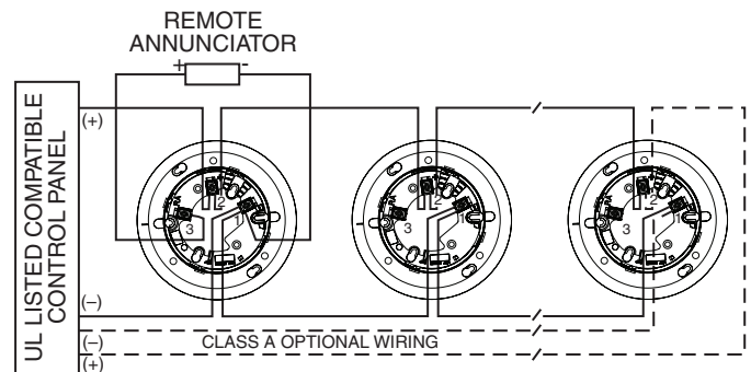
FIGURE 1. WIRING DIAGRAM
