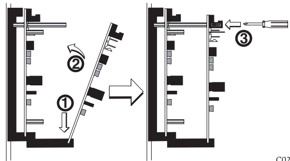
FIGURE 4B. INSTALLATION OF FIK-CZ-6 MODULE IN FRONT CHASSIS POSITION
