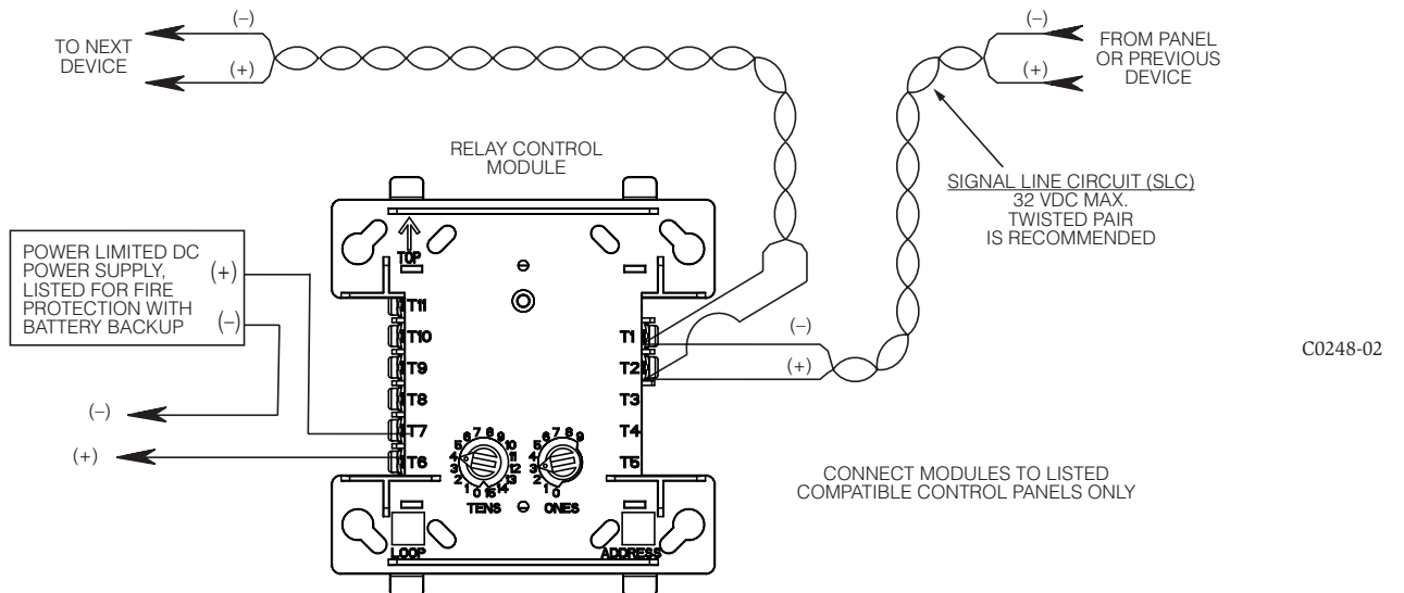
FIGURE 7. RELAY CONTROL MODULE USED TO DISCONNECT A POWER SUPPLY
