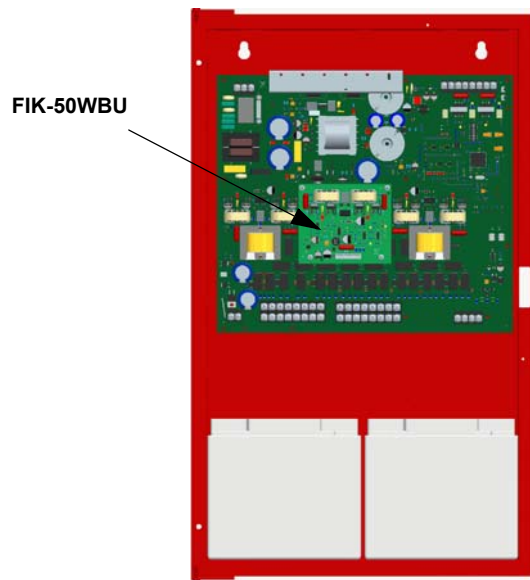
Figure 1 Mounting Location for the FIK-50WBU
