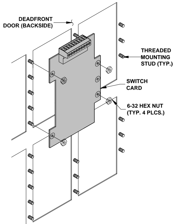
Exhibit 3: Mounting Card to Dead-front Panel
