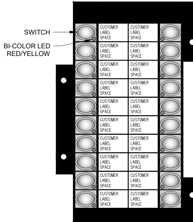
Exhibit 1: Operators View
