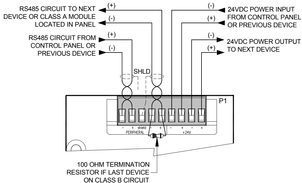
Exhibit 6: Wiring Connections
