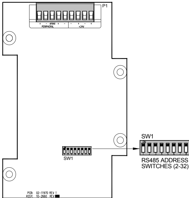
Exhibit 4: Card Addressing
