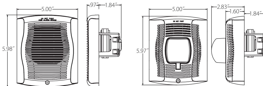
Wall-Mount SP Speaker
