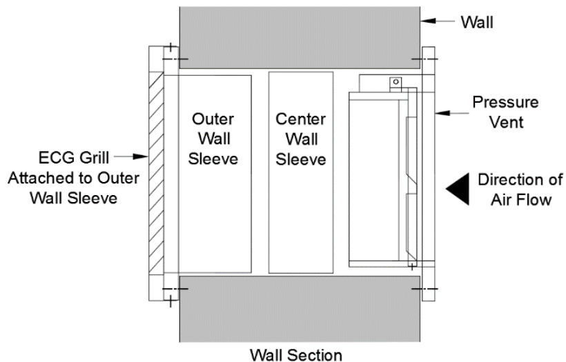
Typical ECG Grill Application
