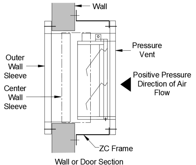
Typical Surface Mounting Frame Application
