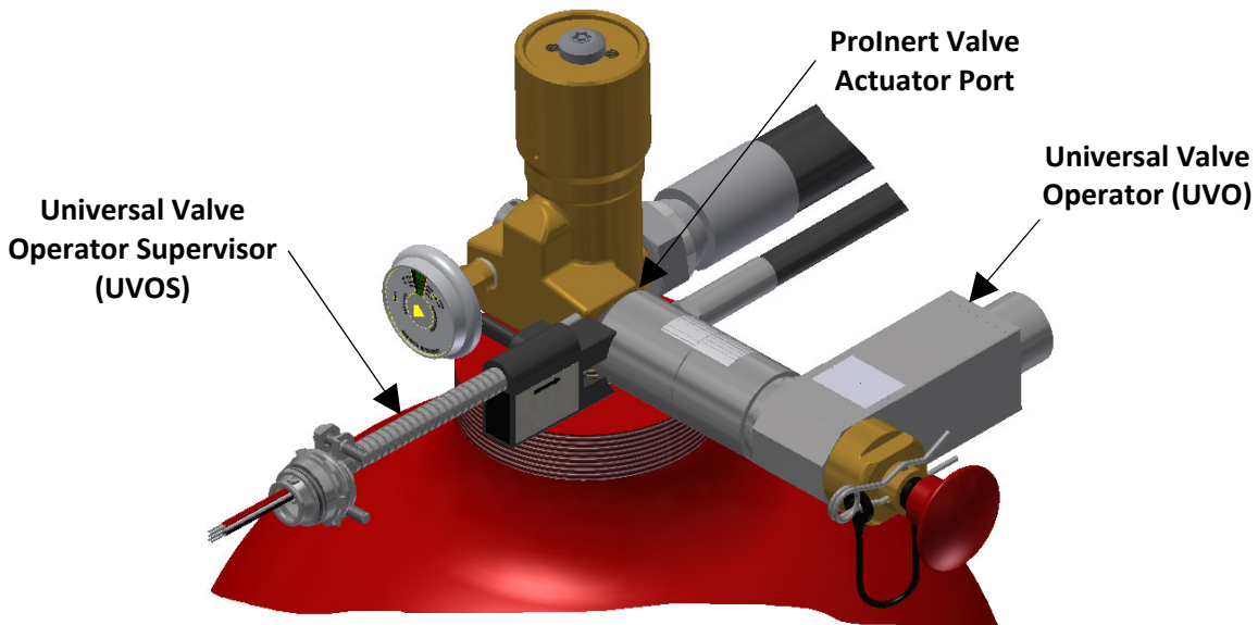
UVOS Installed on Prolnert®2 Cylinder Valve
